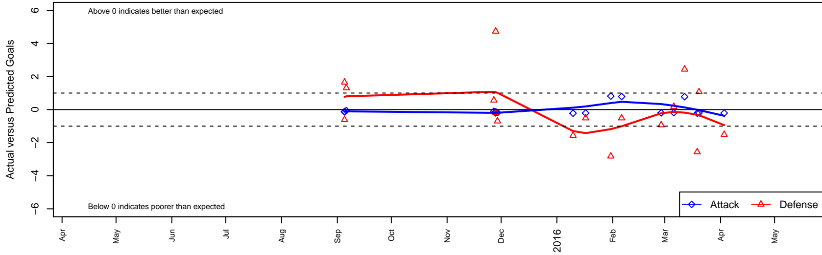
FPSC Fury White G98 Dots are actual minus expected GF (blue circles) and GA (red triangles). Blue line is smoothed change in attack strength. Red is smoothed change in defense strength.
